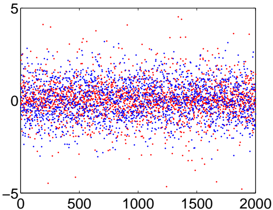
Gaussian v.s. Laplace
