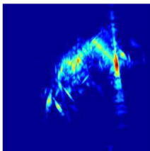
conventional v.s. sparsity
