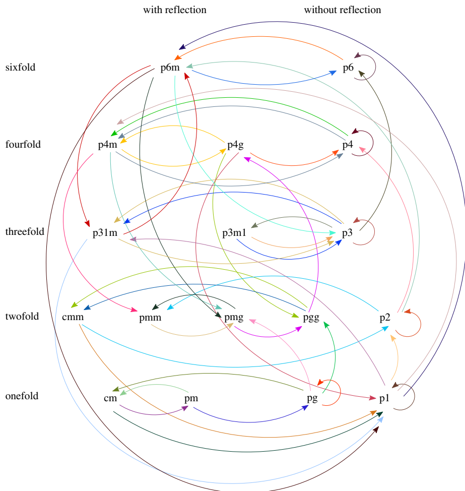
Figure 11. The graph \tilde{\mathcal{G}} of possible group changes observed in the patterns we have identified. The group change of each example pattern considered in this paper is represented using one distinct colour. For instance, the red arrows from p6m to p31m and from p31m to p6m correspond to the p6m \rightarrow p31m \rightarrow p6m standard kagome pattern in figure 1, and the orange arrow from p6 to p6m corresponds to the p6 \rightarrow p6 \rightarrow p6m pattern in figure 1. We remark that \tilde{\mathcal{G}} is only a subgraph of \mathcal{G} , the graph of all possible group changes. (Online version in colour.)
