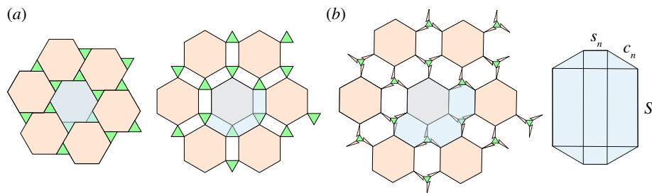
Figure 5. Size change in the triangle–hexagon deployment pattern. (a) The contracted and deployed states of the pattern with no expansion cuts used. The shaded areas represent the unit cell used to calculate the pattern’s size change ratio. (b) On the left, an image of the triangle–hexagon pattern with one round of expansion cuts deployed. On the right, a close-up of an irregular octagon formed by deployment of the expansion cuts. The octagon is broken into the smaller triangles and rectangles we use to determine its area. (Online version in colour.)
