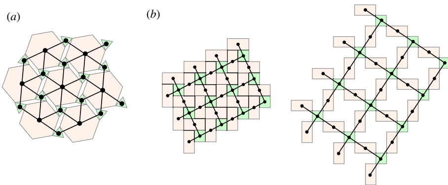
Figure 10. More deployable lattice structures. (a) The topology of the p6 pattern in figure 1 is a deployable (3, 6, 3) lattice. (b) The topology of the p4g and p4 patterns in figure 2n,o is a deployable (2, 4, 2) lattice. (Online version in colour.)
