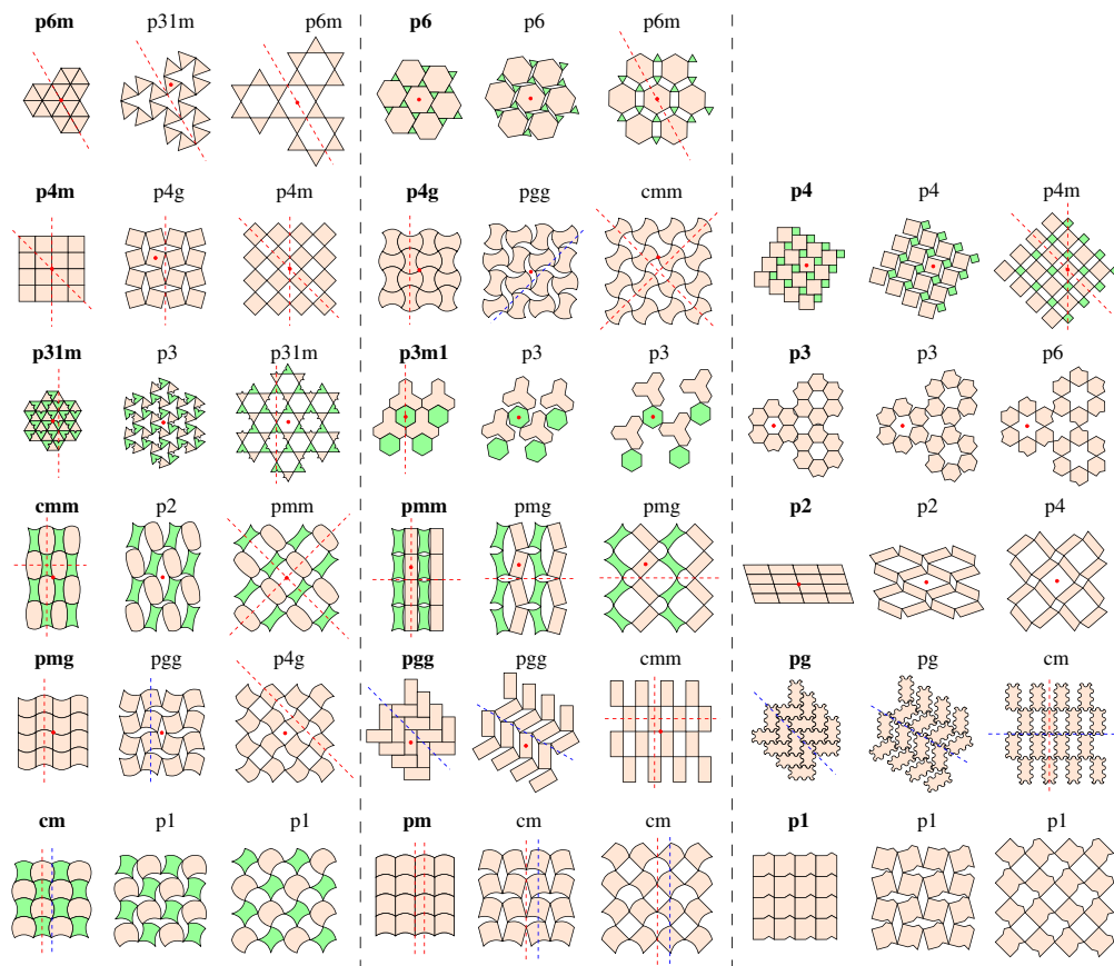
Figure 1. Examples of periodic deployable kirigami patterns in the 17 wallpaper groups. For each example (with the crystallographic notation in bold), we show a portion of the initial contracted state, an intermediate deployed state and the fully deployed state. Tiles with different shapes are in different colours. Key reflection axes (red dotted lines), glide reflection axes (blue dotted lines) and rotation centres (red dots) that can be used for determining their wallpaper group type are highlighted. (Online version in colour.)
