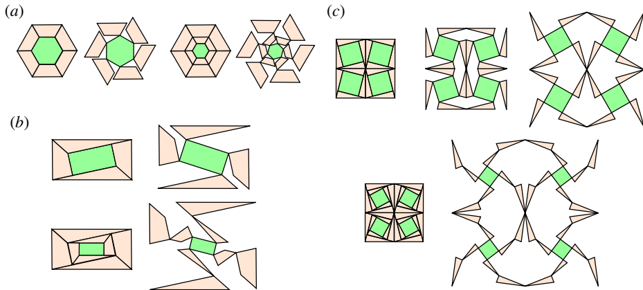
Figure 4. More symmetry-preserving expansion cut patterns. (a) An expansion cut pattern that can be introduced on any tile with sixfold rotational symmetry. The cut pattern achieves an expansion throughout deployment while preserving the sixfold symmetry of the tile. (b) An expansion cut pattern that can be introduced on any tile with twofold rotational symmetry. The cut pattern achieves an expansion throughout deployment while preserving the twofold symmetry of the tile. (c) An expansion cut pattern with twofold rotational symmetry that preserves both the rotational symmetry and reflectional symmetry. The expansion cut pattern is derived from the pattern in figure 3 a with four copies of it placed appropriately to form a pattern that preserves the reflectional symmetry throughout the deployment. The top row shows the deployment of the pattern with one level of cuts. The bottom row shows the deployment of the pattern with two levels of cuts. (Online version in colour.)
