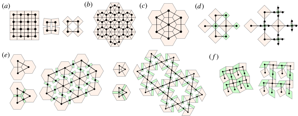
Figure 9. Lattice representations of kirigami patterns. (a) The regular (4, 4) lattice representing the standard quad topology (e.g. the p4m, p4g, pmg patterns in figure 1), with each tile connected to exactly four adjacent tiles. (b) The regular (3, 3) lattice representing the standard kagome topology (e.g. the p6m, p3m1 and p3 patterns in figure 1). (c) The regular (6, 6) lattice. Note that the triangles in it make the structure rigid. (d) Using the expansion cuts introduced in figure 3, we can turn a deployable structure with the regular (4, 4) lattice into another deployable structure with a (2, 4, 2) lattice. (e) Using the expansion tiles introduced in figure 3, we can turn the triangles in a rigid lattice into another polygon, thereby producing novel deployable patterns with a (2, 6, 2) lattice (left) or a (2, 4, 2) lattice (right). Both examples shown here are p6m \rightarrow p6 \rightarrow p6 . (f) Breaking certain connections in a given lattice yields a onefold deployable structure with another lattice representation. The example shown here is a p4g \rightarrow p1 \rightarrow p1 pattern with a (1, 3, 4, 3, 1) lattice (see also the p31m pattern in figure 6f with a (2, 4, 4, 2) lattice). (Online version in colour.)
