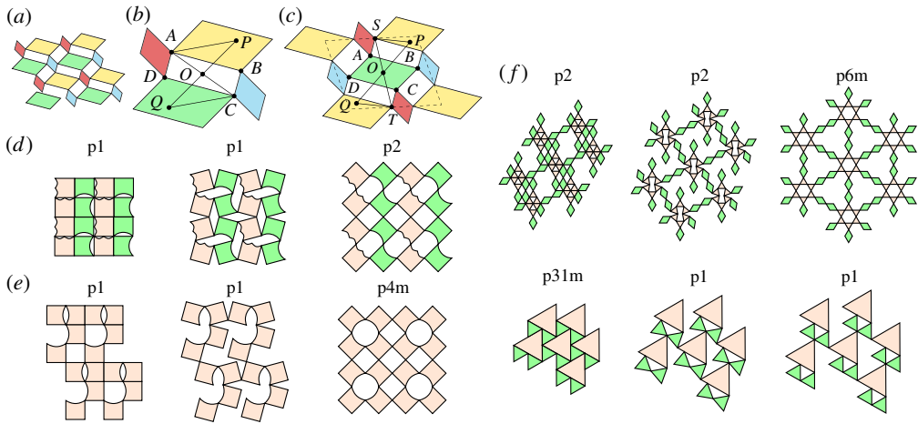
Figure 6. Exploring possible symmetry changes. (a) A general deployed quad pattern with twofold rotational symmetry. The parallelograms can be changed in pairs (red and blue or yellow and green) to other shapes whose vertices form parallelograms. (b) For the case where the centre of rotation (COR) O is at the centre of a rift (i.e. a gap that forms when tiles separate during deployment) in the deployed state, consider two corresponding points P, Q within tiles and denote the two opposite vertices of the rift by A and C . We can show that \triangle APO \cong \triangle CQO throughout deployment or contraction, which implies that the contracted pattern is also with twofold rotational symmetry. (c) For the case where the COR O is at the centre of a tile. We remark that the pattern here should not be thought of as a supercell of b ; the parallelograms are just used for simplicity to represent the tiles and can be changed to other shapes. However, whether a COR is at the centre of either a tile or a rift depends on the tile shapes. (d) For the case where the COR O is at the intersection point of two tiles, we construct a deployable pattern that achieves a onefold to twofold symmetry change. (e) Using a variation of the standard quad kirigami topology, we can achieve a onefold to fourfold symmetry change as well as a gain in reflection. (f) Introducing floppiness can lead to a large variety of symmetry changes, such as a twofold to sixfold symmetry gain ( p2 \rightarrow p2 \rightarrow p6m ) or a loss in all symmetries ( p31m \rightarrow p1 \rightarrow p1 ). For each pattern, tiles with different shapes are in different colours. (Online version in colour.)
