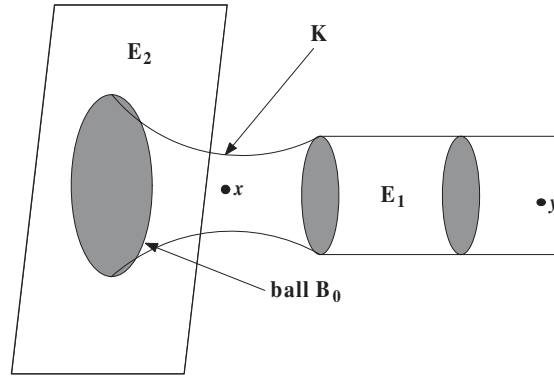
FIGURE 3.1. M = E_1 \cup E_2 \cup K .
