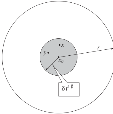
FIGURE 4.1. Balls B(x_0, r) and B(x_0, \delta t^{1/\beta}) .
